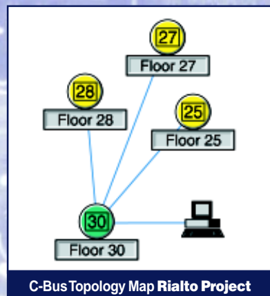
Network Topology showing C-Bus Network for Rialto.
